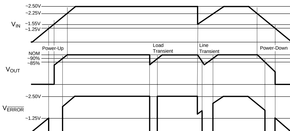
Figure 5. \overline{ERROR} Flag when Pull-Up is from V_{IN}
