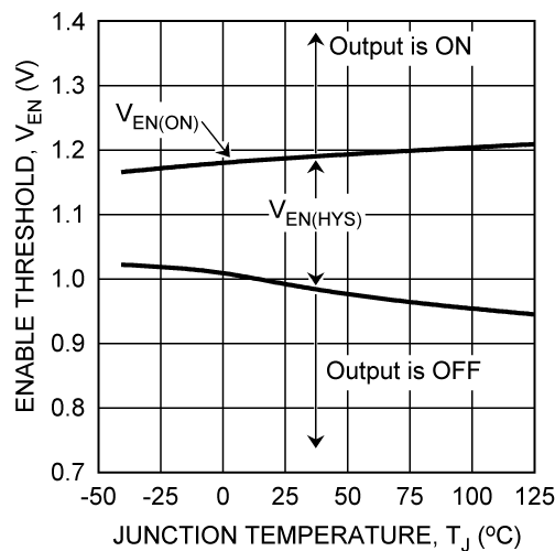
Figure 2. Enable Threshold
