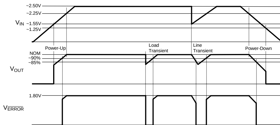
Figure 4. \overline{ERROR} Flag when Pull-Up is from V_{OUT}
